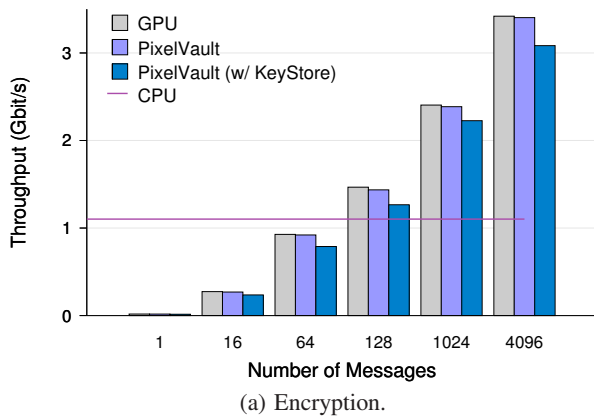
(a) Encryption.
