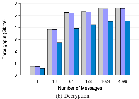
(b) Decryption.
